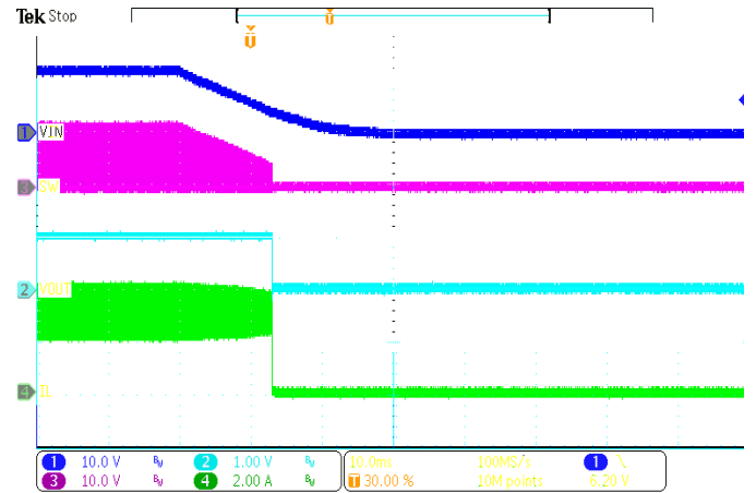
Figure 9. Power Down
