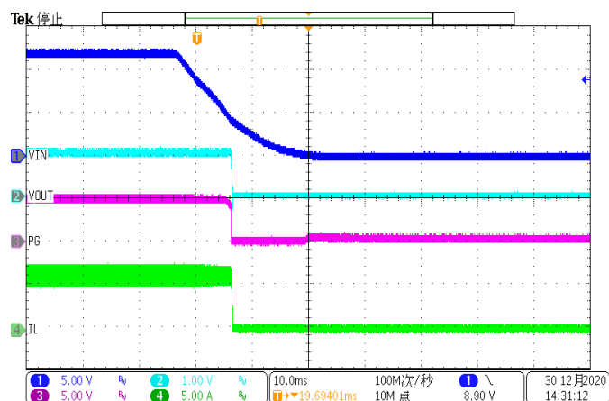
Figure 12. Power down
