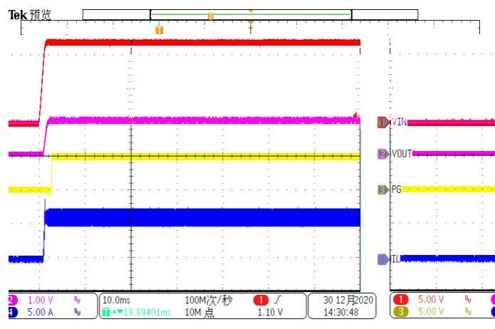
Figure 11. Power up
