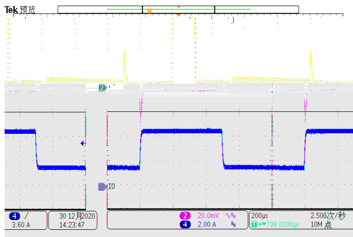
Figure 17. Load Transient (1.5A-4.5A, 1.6A/us)
