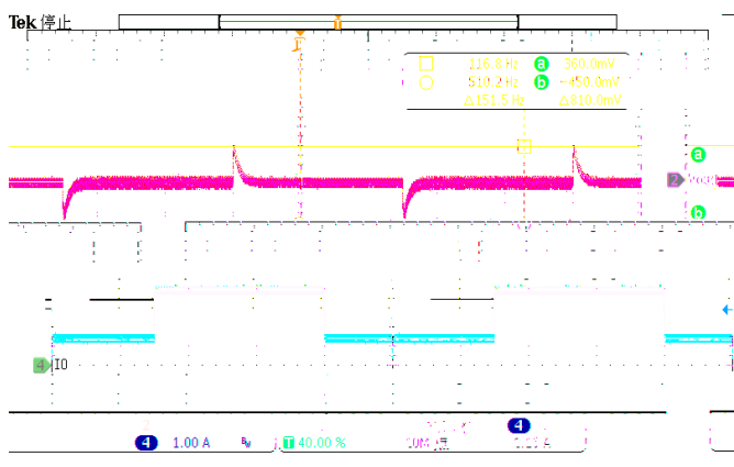
Figure 35. LoadTrans (Iload=0.5A-1.5A)
