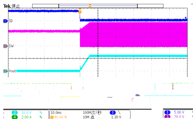
Figure 34. Shutdown remove
