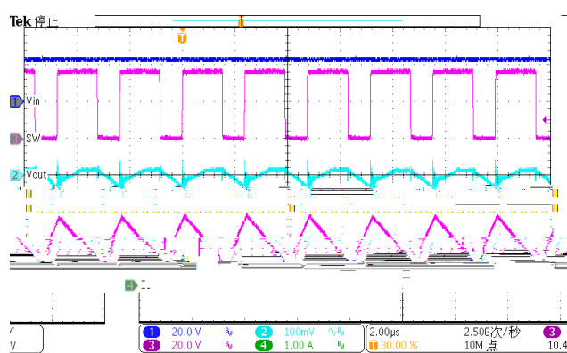
Figure 36. steady-state (Iload=2A)
